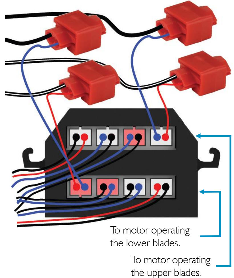
Dual motor Powerlouvre Gallery set
